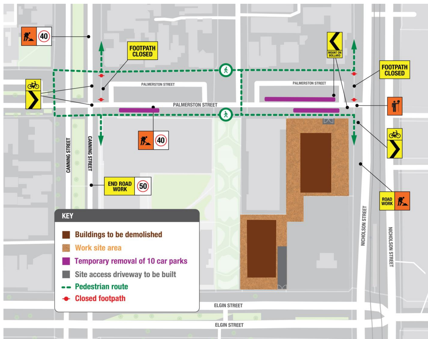
Image 1: Elgin Towers, traffic management and work site set up
